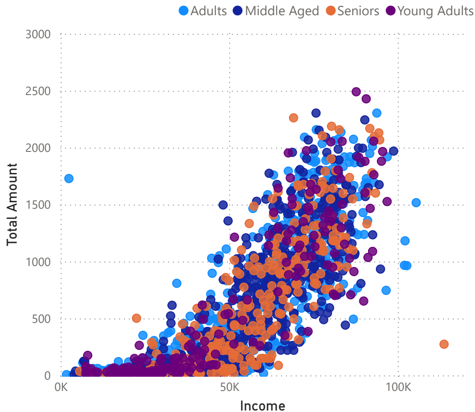
Income vs Spending
