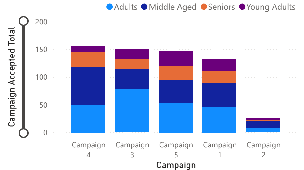
Campaign Acceptance by Age Groups
